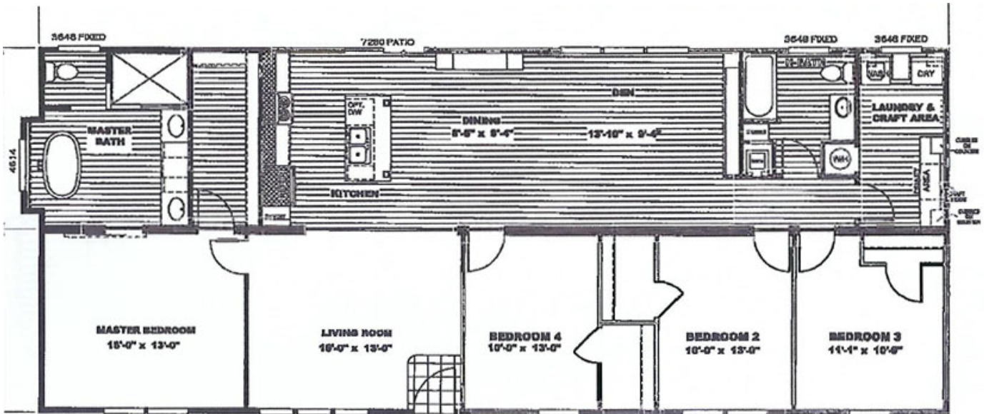
MODEL: "The Patriot" #33 28 x 68 (72' overall) 4 Bedroom, 2 Bath
